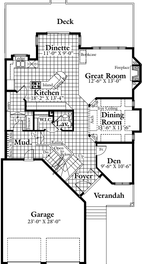
MAIN FLOOR PLAN 1270 SQ.FT.
