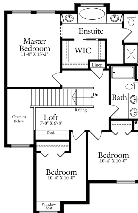
Main Floor Plan 890 SQ.FT.
