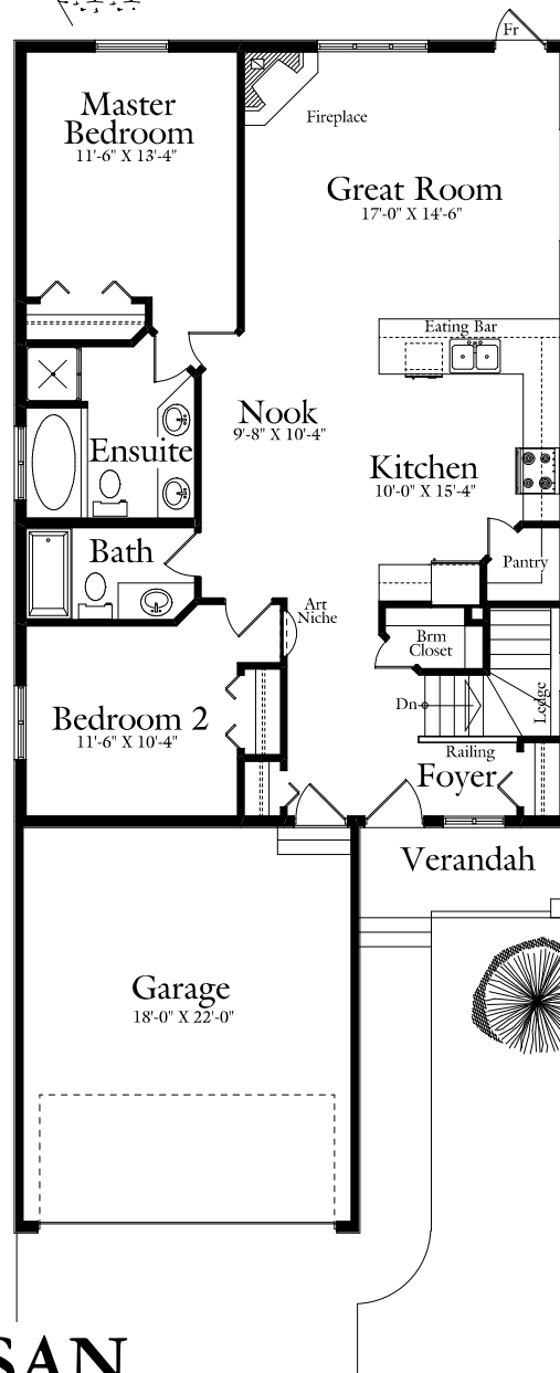
Main Floor Plan 1275 SQ.FT.
